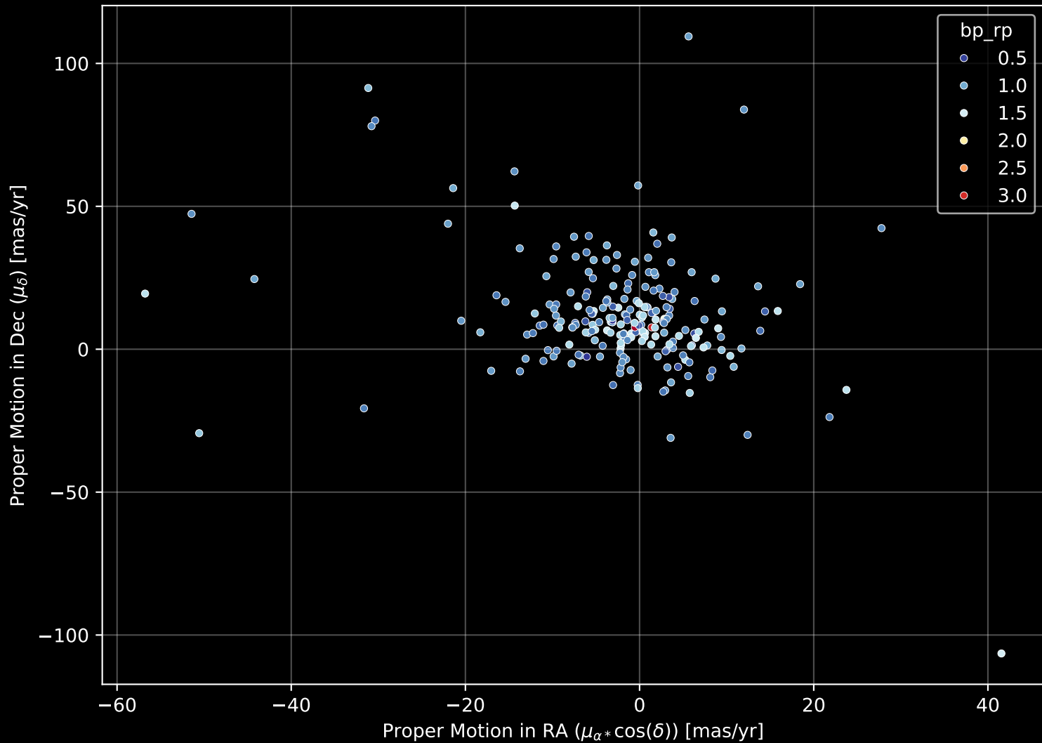
GALAH DR4 Field: [7201] Proper Motion Diagram (n= 226)
