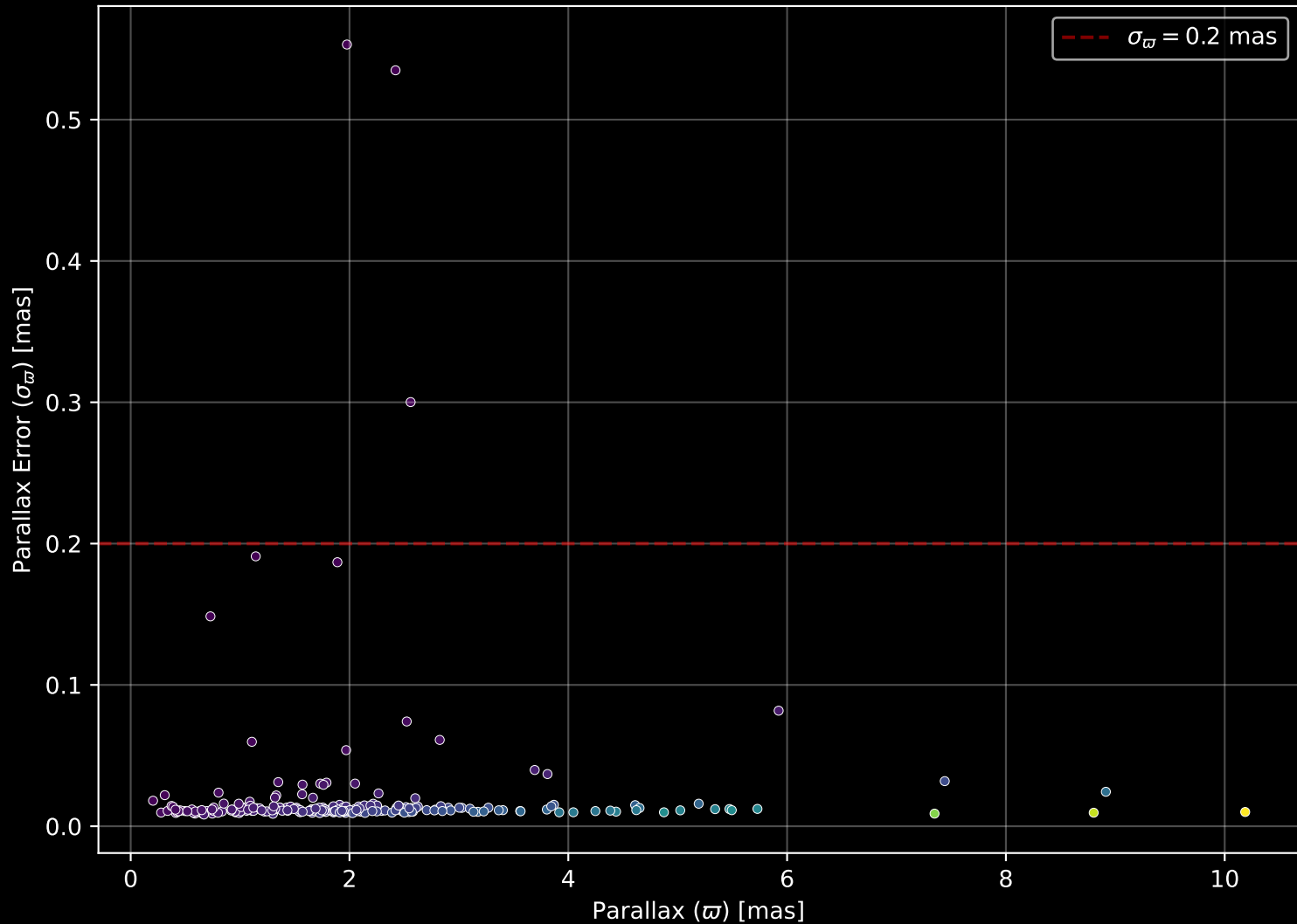
GALAH DR4 Field: [7201] Parallax Quality (n= 226)
