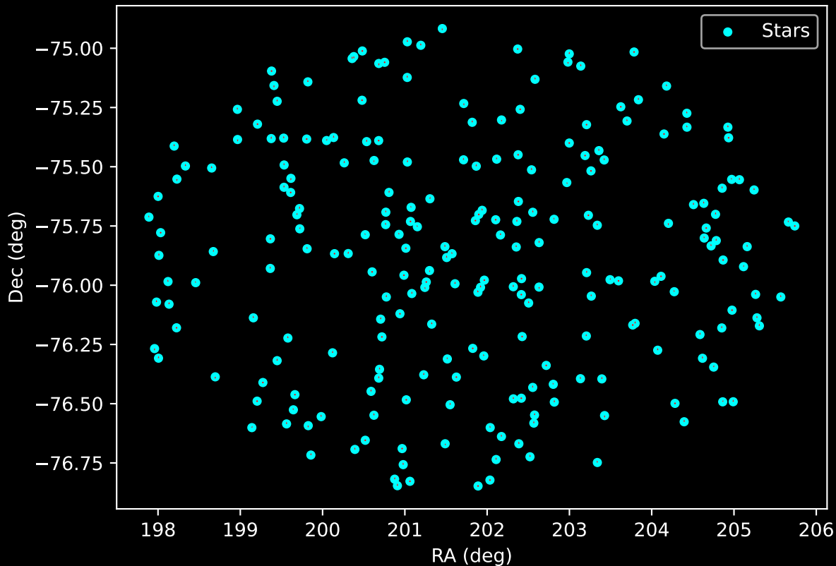
GALAH DR4 Field: [7201] Proper Motion Vectors for Gaia Star Field (n= 226)
