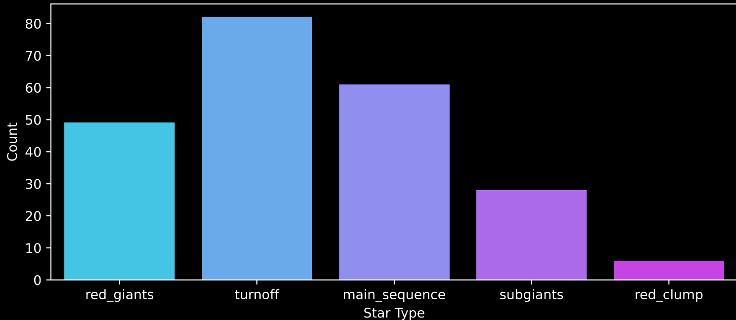
GALAH DR4 Field: [7201] Count plot of Star Type
