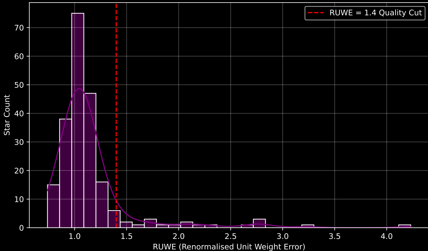
GALAH DR4 Field [7201] RUWE Distribution (n= 215)
